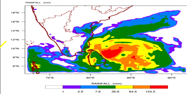
WRF-RegGSI MODEL FORECAST (24 HR.) RAINFALL (mm) based on 00 UTC of 29-10-2012 valid for 03 UTC of 30-10-2012
